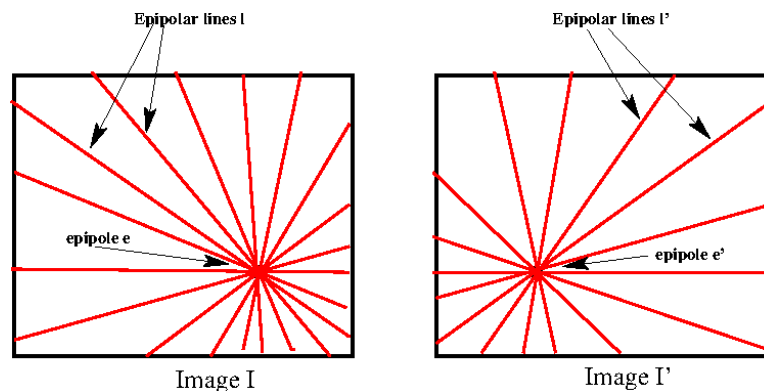
Figure 2: Epipolar Lines
