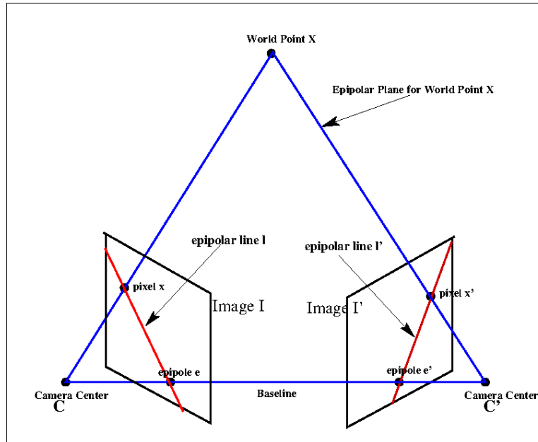
Figure 1: Epipolar Geometry
