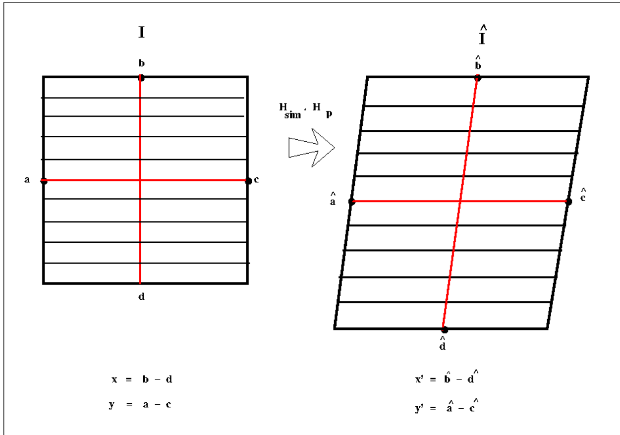
Figure 4: Defining the “a-c” and “b-d” vectors for the Shearing Homography
