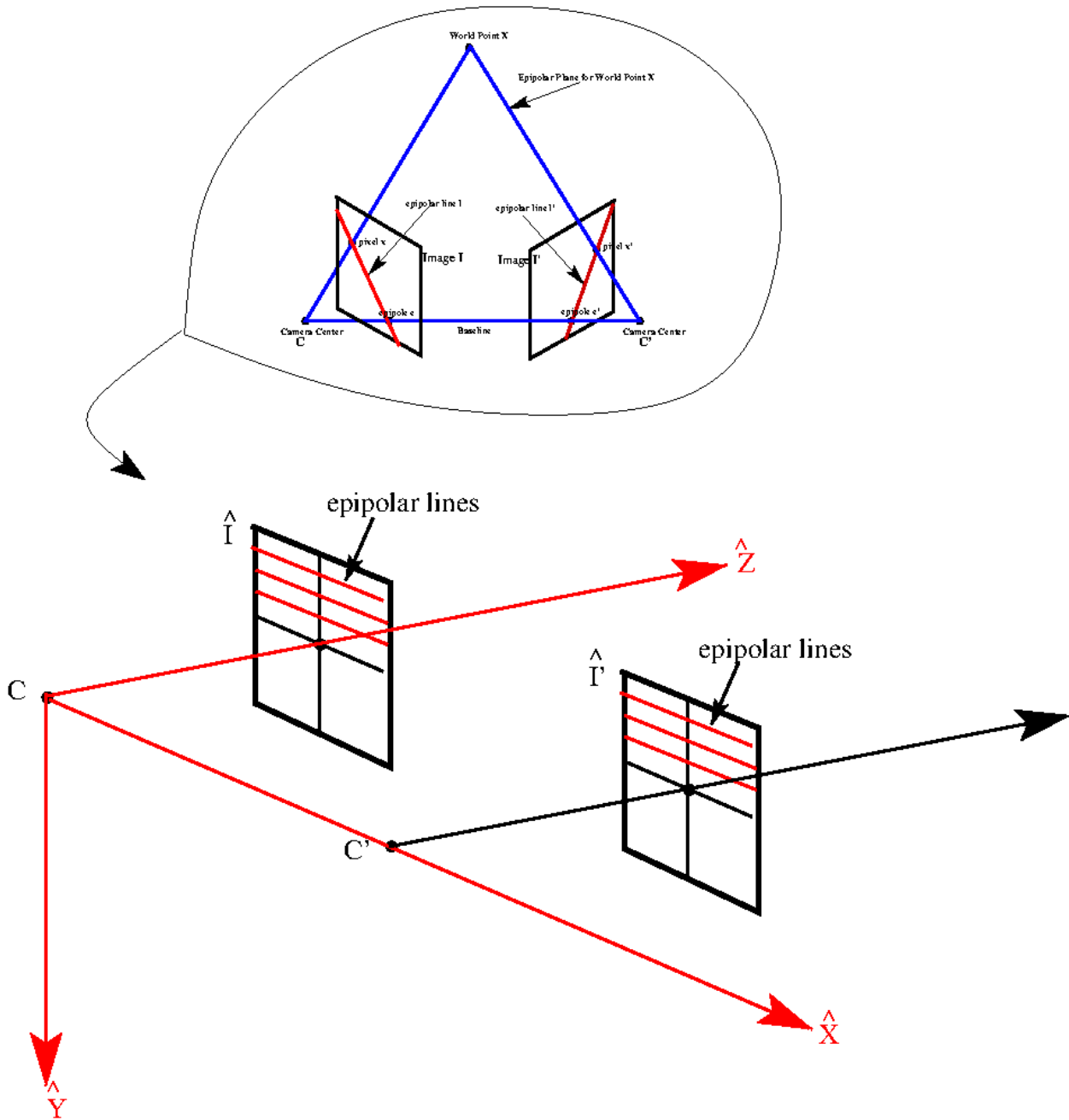
Figure 3: Stereo Rectification: The original image pair in the bubble: (I, I') and the rectified image pair (\hat{I}, \hat{I}')
